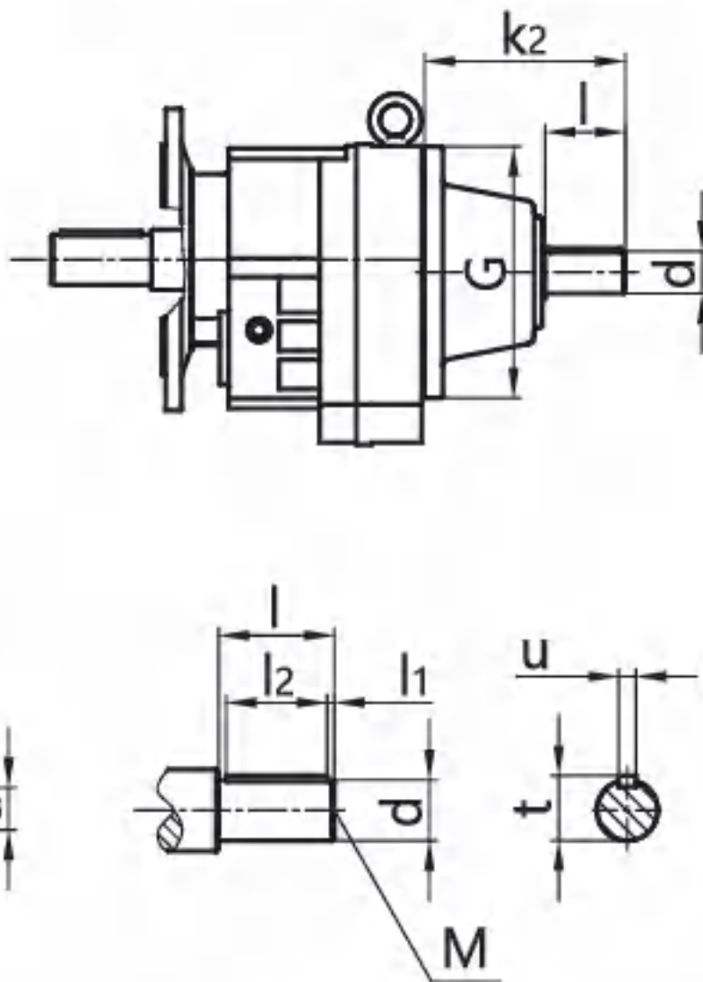
GR..29-179AD1-8 Mounting Dimensional Description
