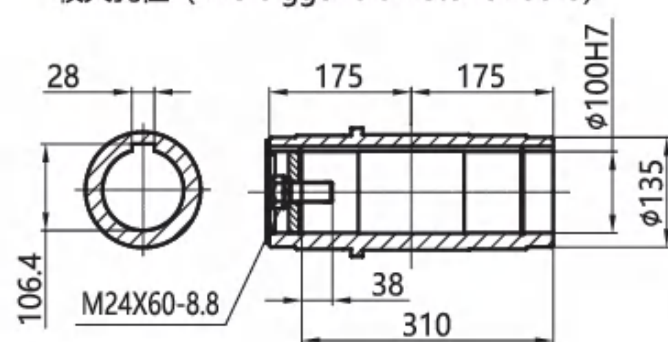
较大孔径 (The bigger diameter of bore)
