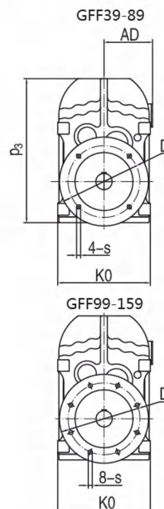
GFF39-159 Mounting Dimensional Description
