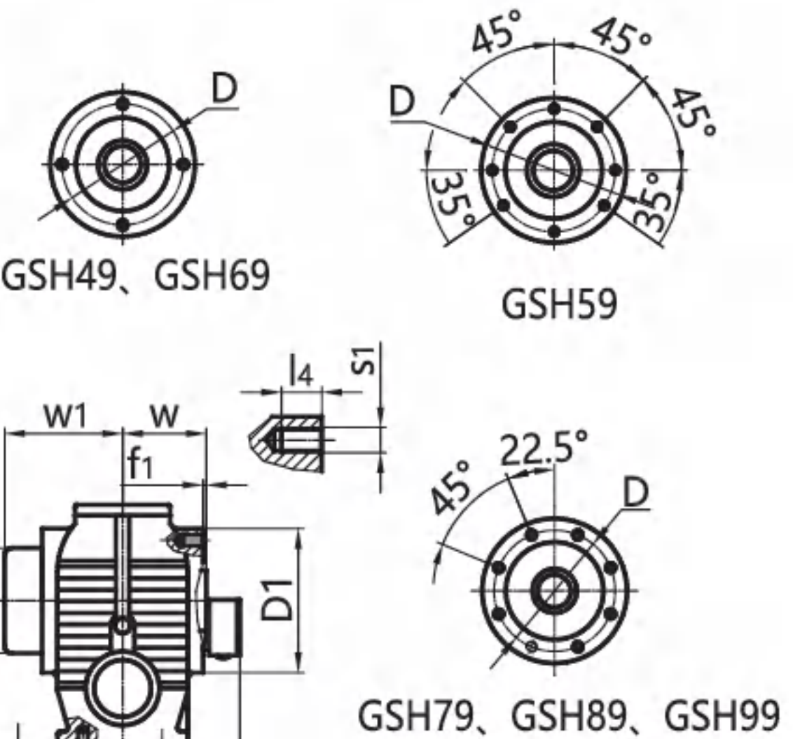
GSH49-99 Mounting Dimensional Description
